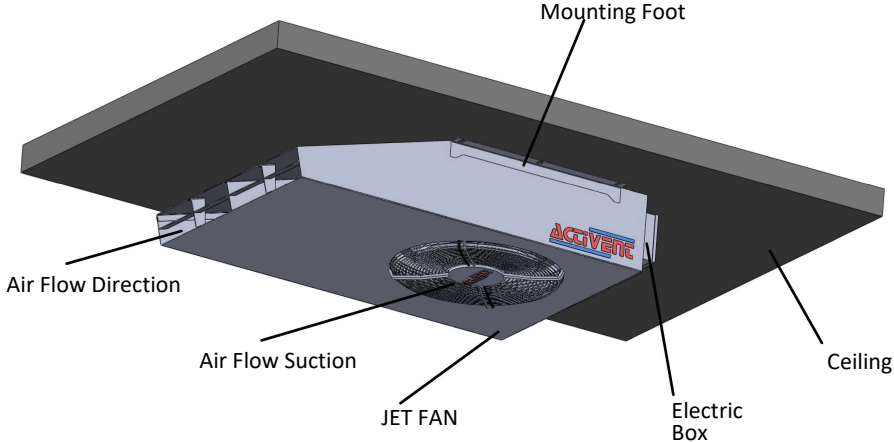
Radial Jet Fan Ceiling Mounting Detail
