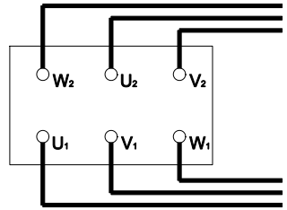
Y/Δ Connection
