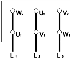
Δ Connection
