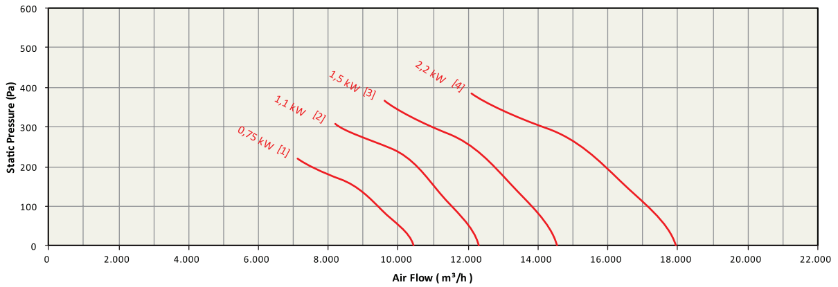
[1]: AKPP-630-1,00-T-4K [2]: AKPP-630-1,50-T-4K [3]: AKPP-630-2,00-T-4K [4]: AKPP-630-3,00-T-4K
