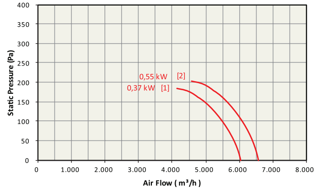
[1]: AKPP-450-0,50-T-4K [2]: AKPP-450-0,75-T-4K
