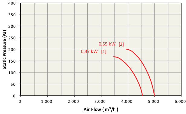
[1]: AKPP-400-0,50-T-4K [2]: AKPP-400-0,75-T-4K
