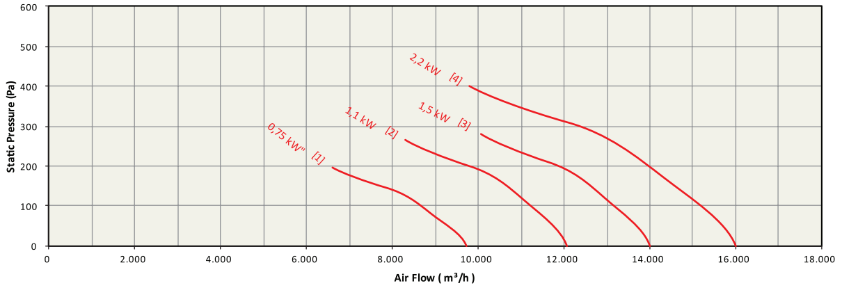
[1]: AKPP-560-1,00-T-4K [2]: AKPP-560-1,50-T-4K [3]: AKPP-560-2,00-T-4K [4]: AKPP-560-3,00-T-4K
